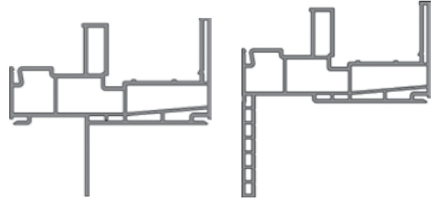
1-3/8" Nail-Fin for New Construction Openings
